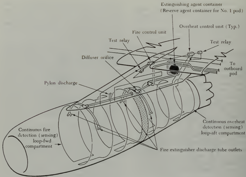
FIGURE 9-10. Typical pod and pylon fire protection installation.
